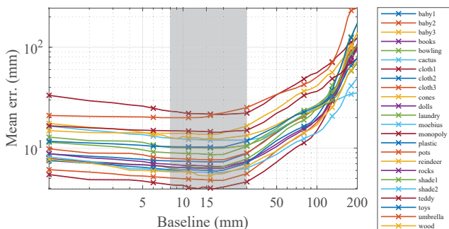
Figure 4: Accuracy of MSL vs. baseline. The plot shows accuracy of MSL vs. baseline using simulations on a few example scenes from the Middlebury dataset. Across scenes, MSL achieves the best performance with a baseline from 8 to 30mm.
